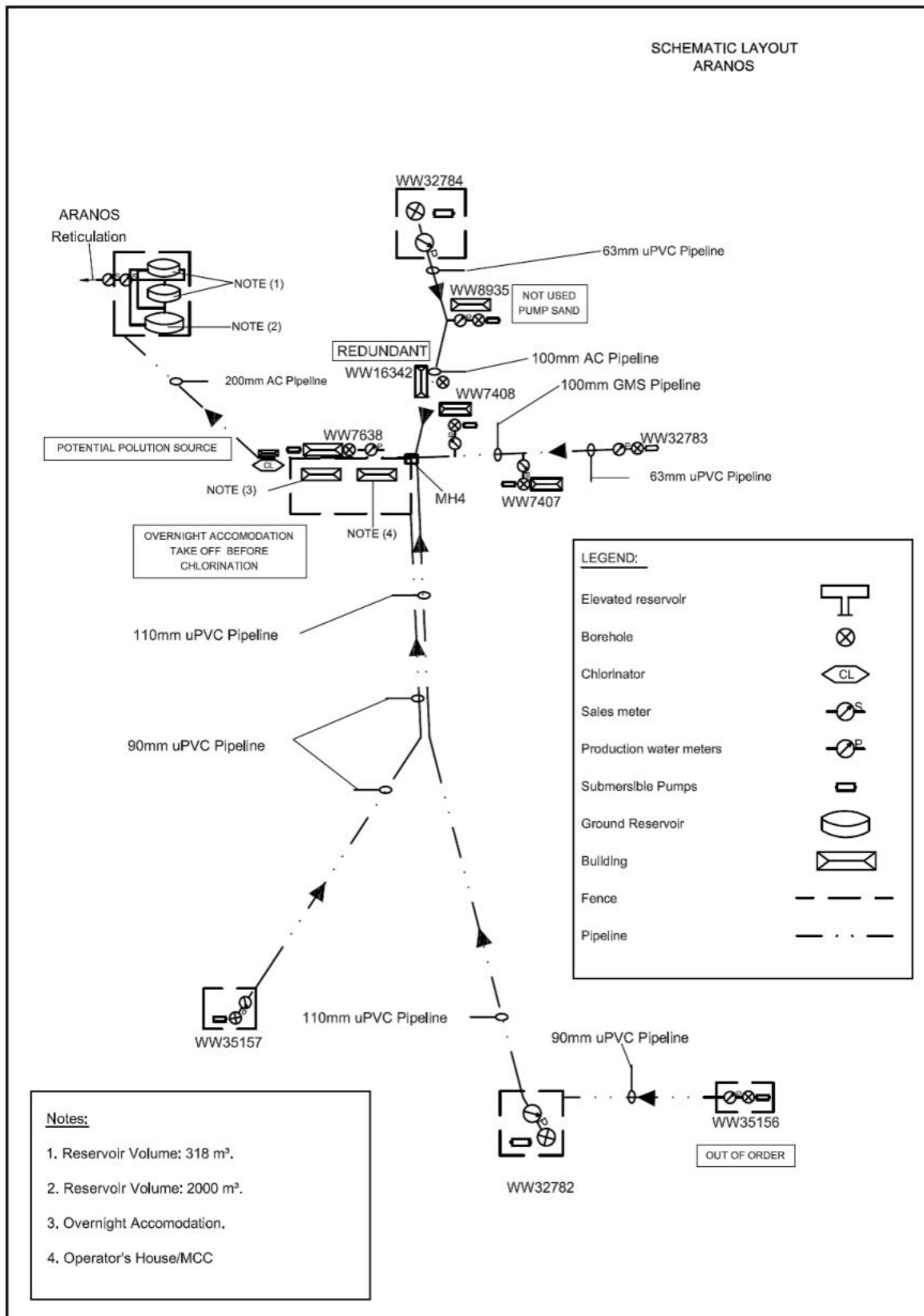
Figure 2: Aranos Scheme Schematic
