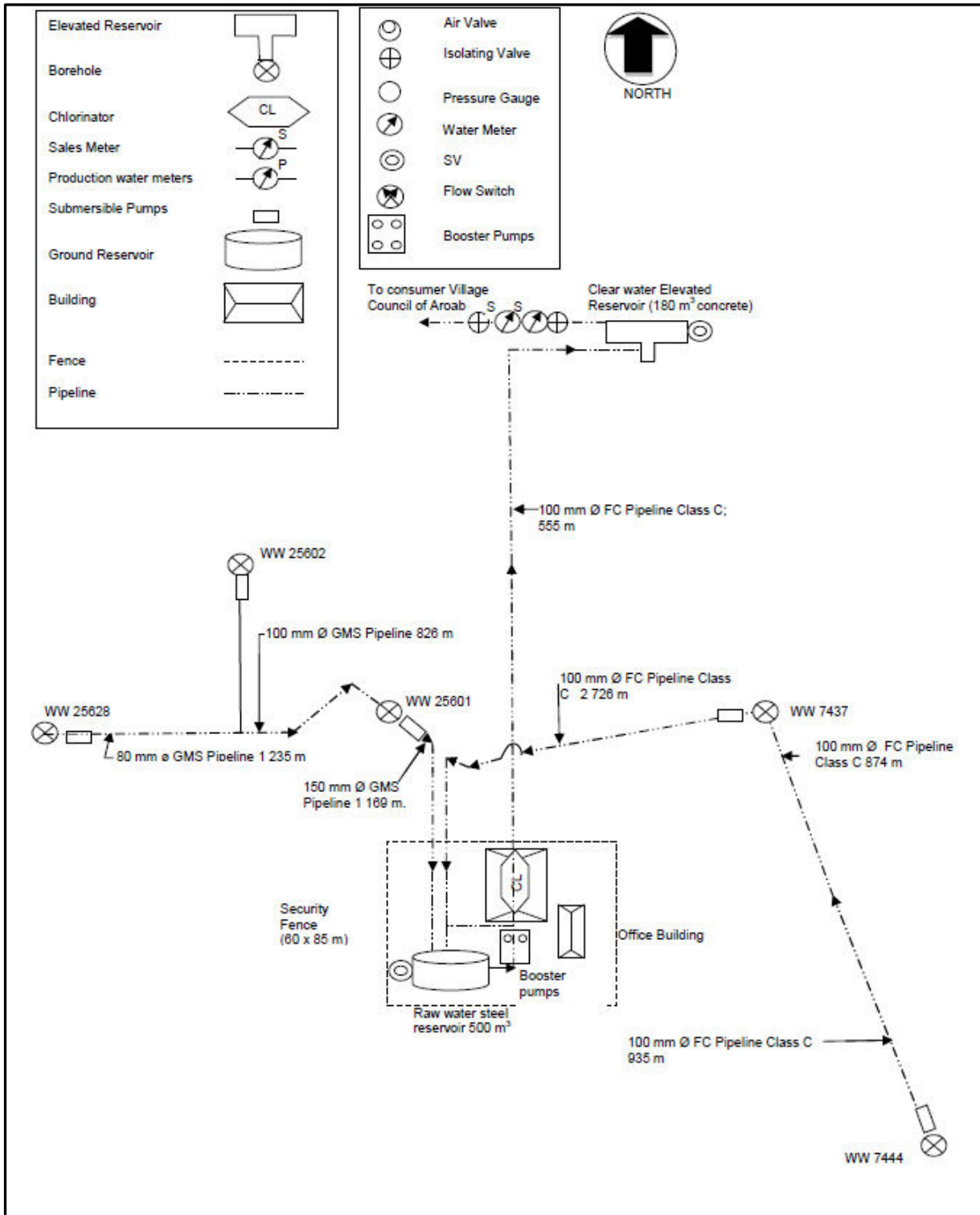
Figure 1: Aroab Scheme Schematic Layout
