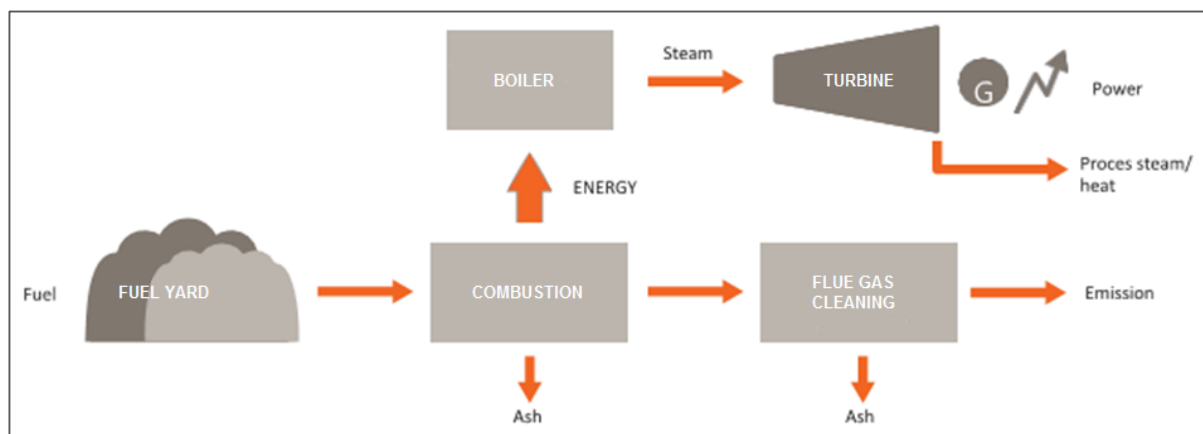
FIGURE 2 TYPICAL CONFIGURATION OF A BIOMASS COMBUSTION PLANT
