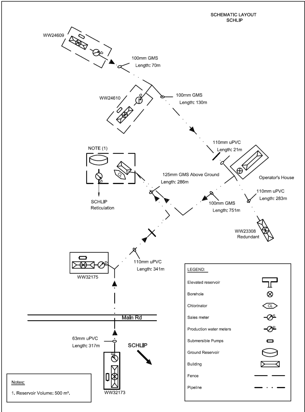
Figure 2: Schlip Scheme Schematic Layout
