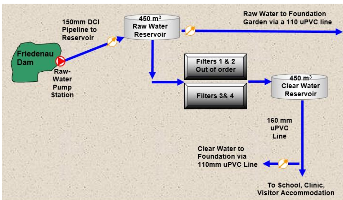
Figure 2: Baumgartsbrunn Scheme Schematic Layout
