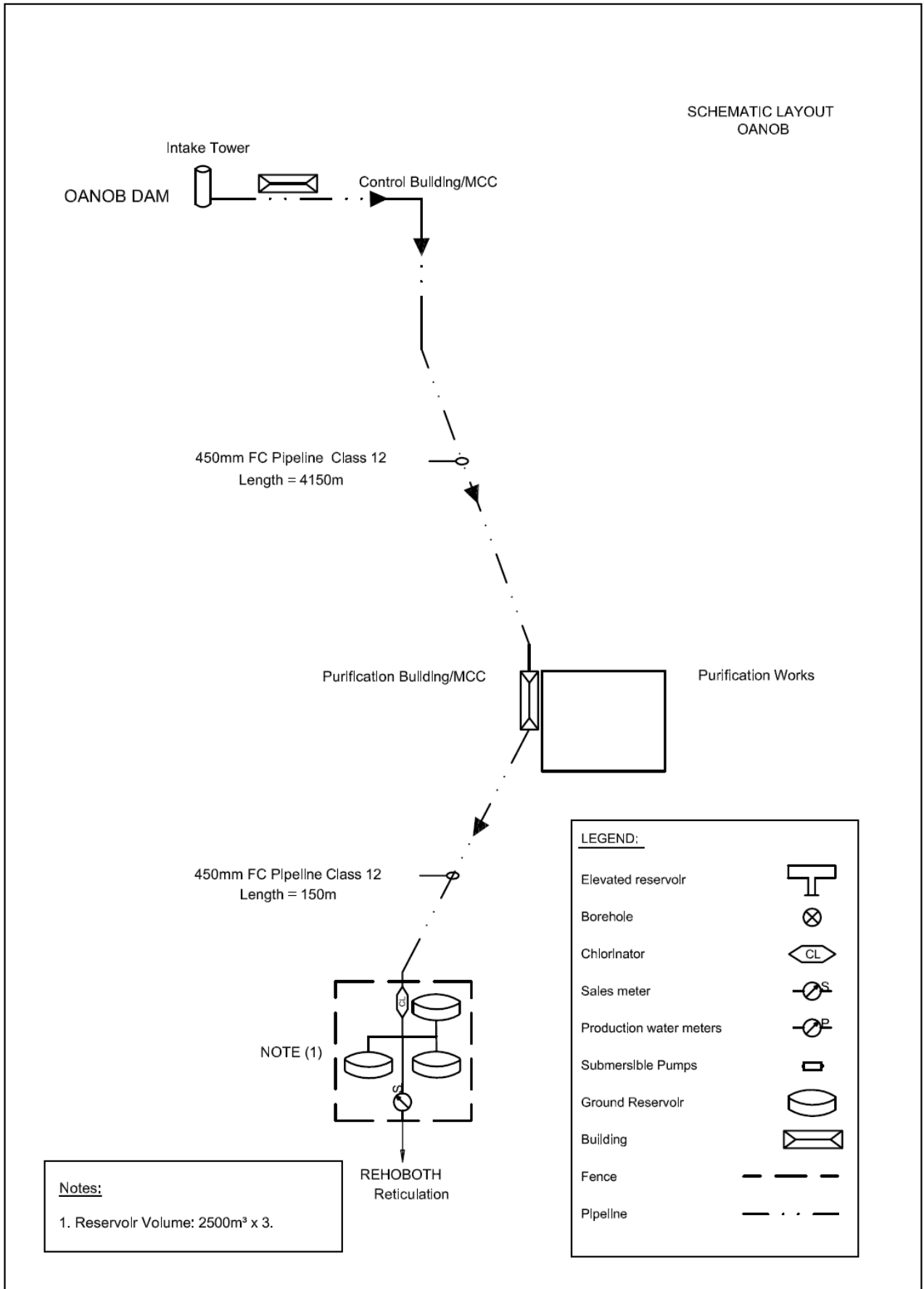
Figure 2: Rehoboth Town-Oanob Dam Scheme Schematic Layout
