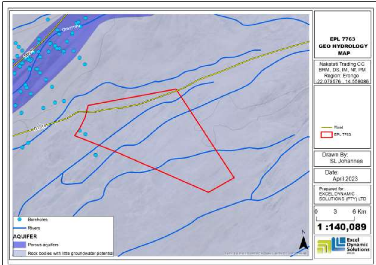
Figure 8: Shows groundwater map for the project area
