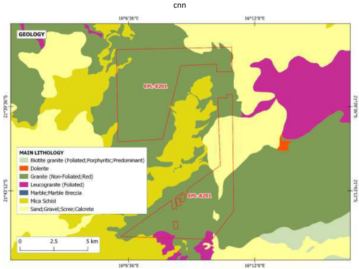
Figure 5: The geology of the EPL
