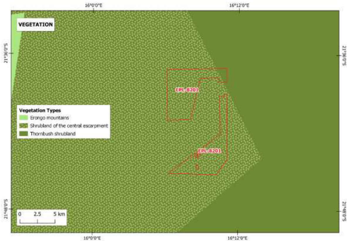
Figure 8: Vegetation Cover for EPL 8201
