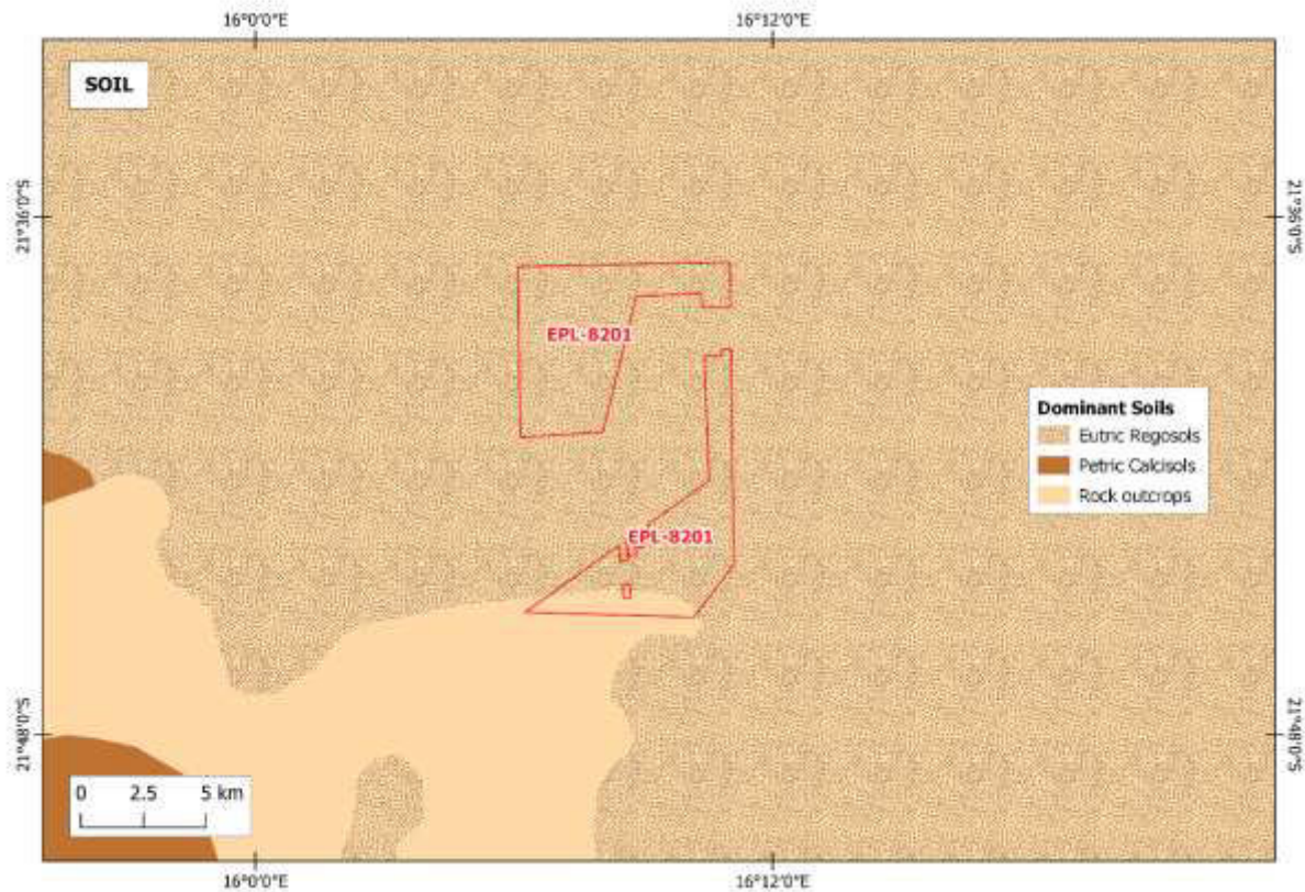
Figure 6: The soils map of the EPL 8201
