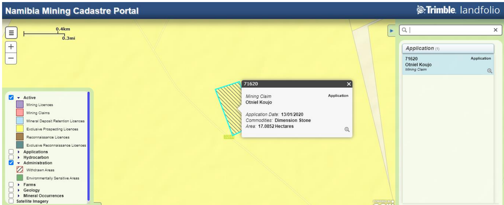
Figure 1: Locality map of the mining claim 71620 at Farm Kompaneno 104, Omaruru Constituency, Erongo Region, located about 23 km off the C36 road onto the D2344 road from Omaruru to Omatjete (-21.2513889°, 15.74777778°). (MME Portal, 2020)
