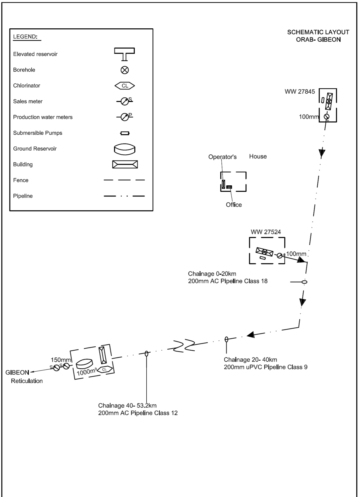
Figure 2: Gibeon Scheme Schematic Layout
