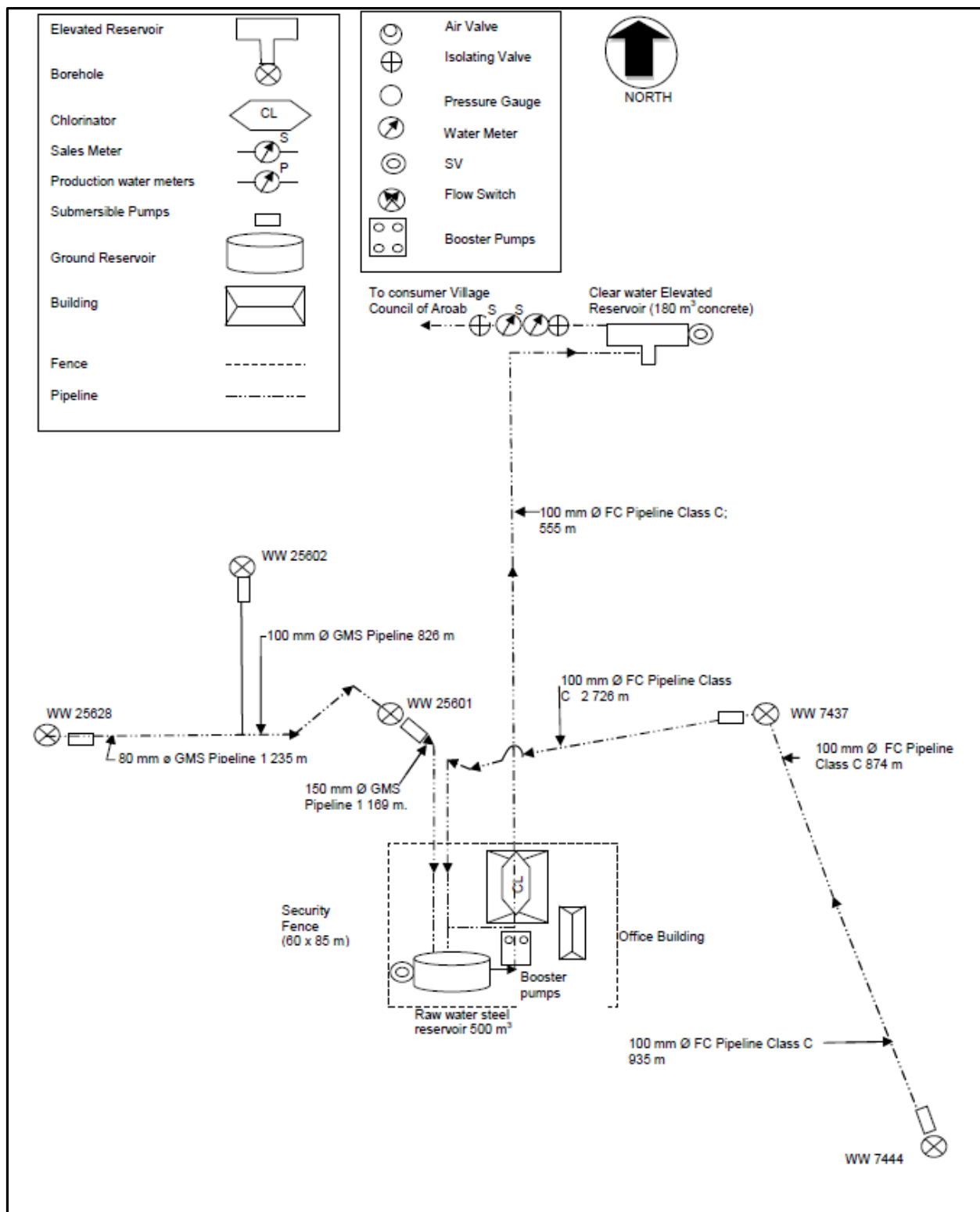
Figure 2: Aroab Scheme Schematic Layout
