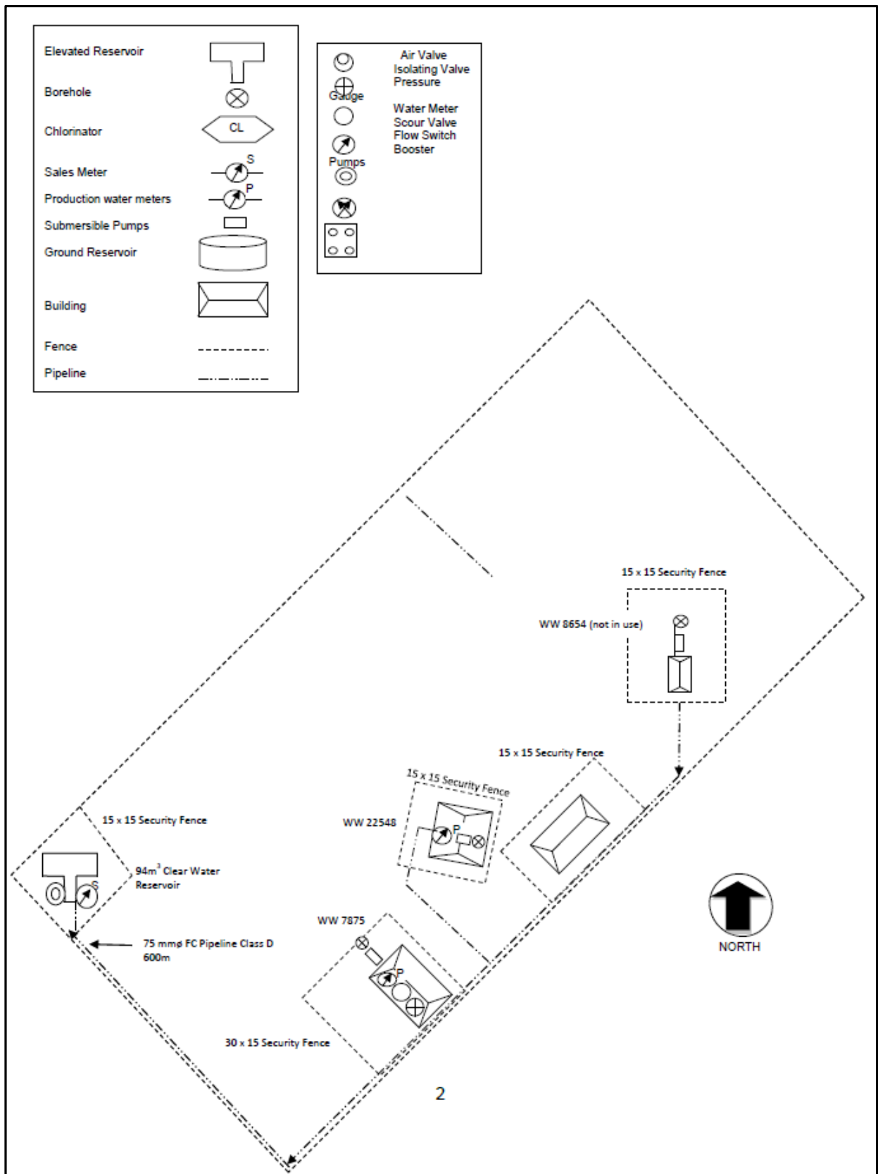
Figure 2: Ariamsvlei Scheme Schematic Layout
