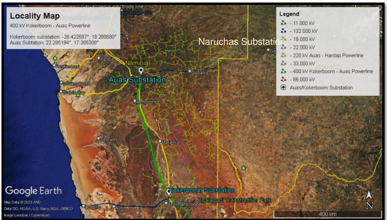
Figure 1: Locality map showing the 400kV Auas – Kokerboom transmission line
