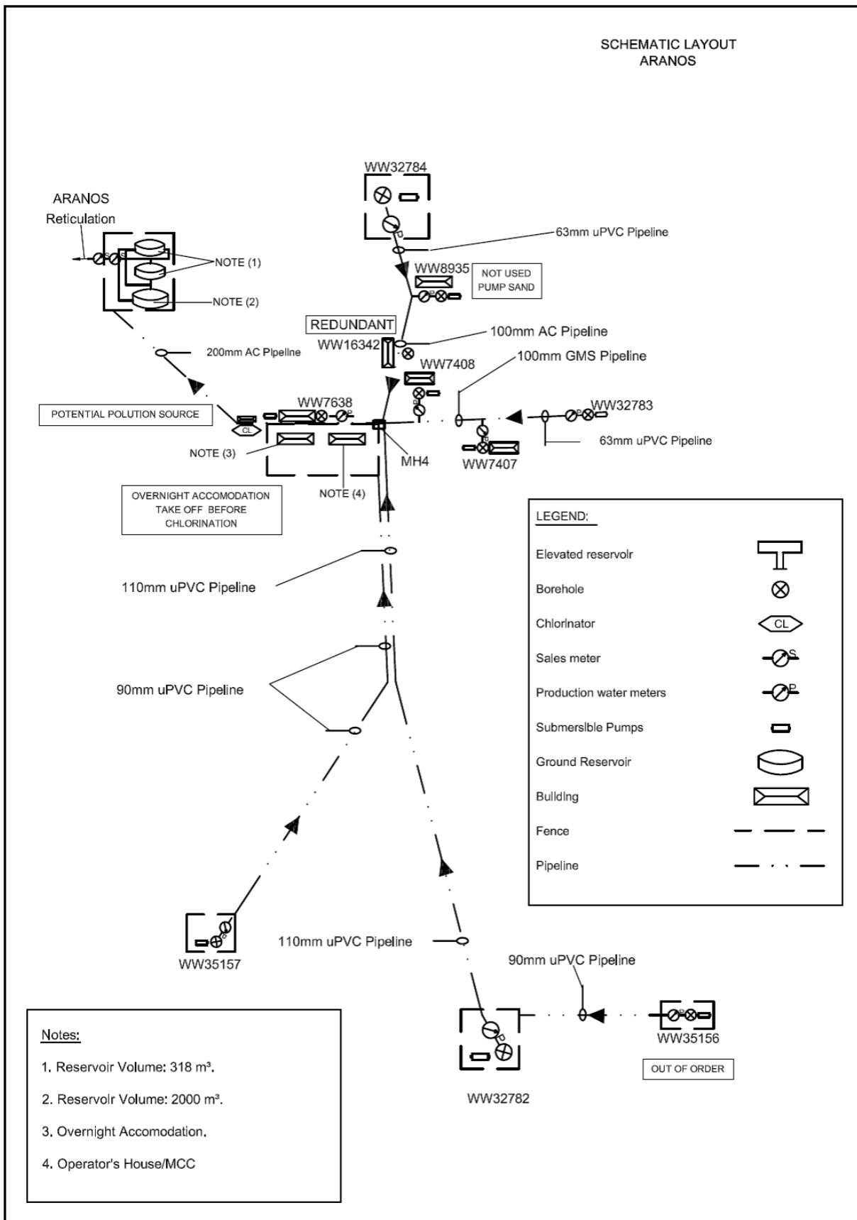
Figure 2: Aranos Scheme Schematic
