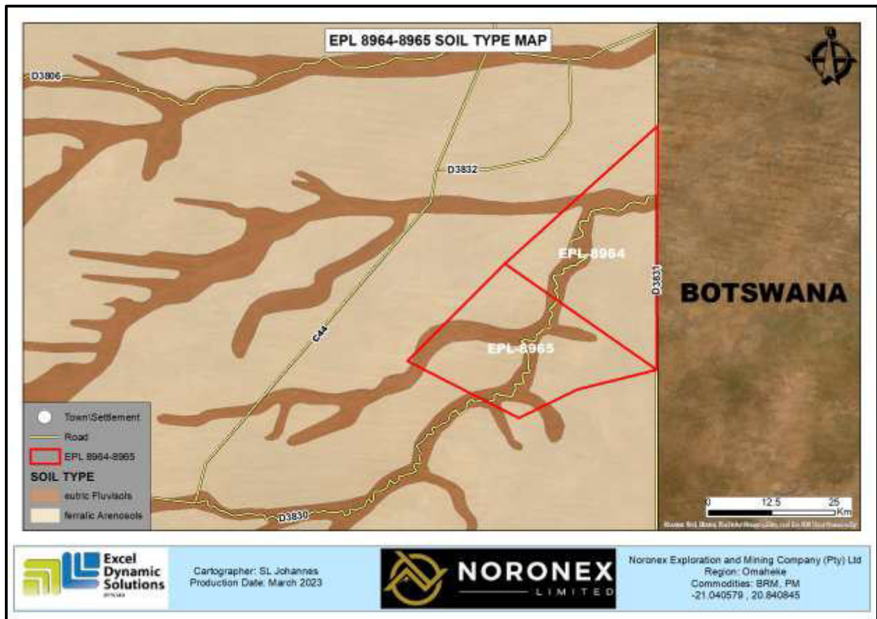
Figure 7: Soils map - EPL 8964 - 8965
