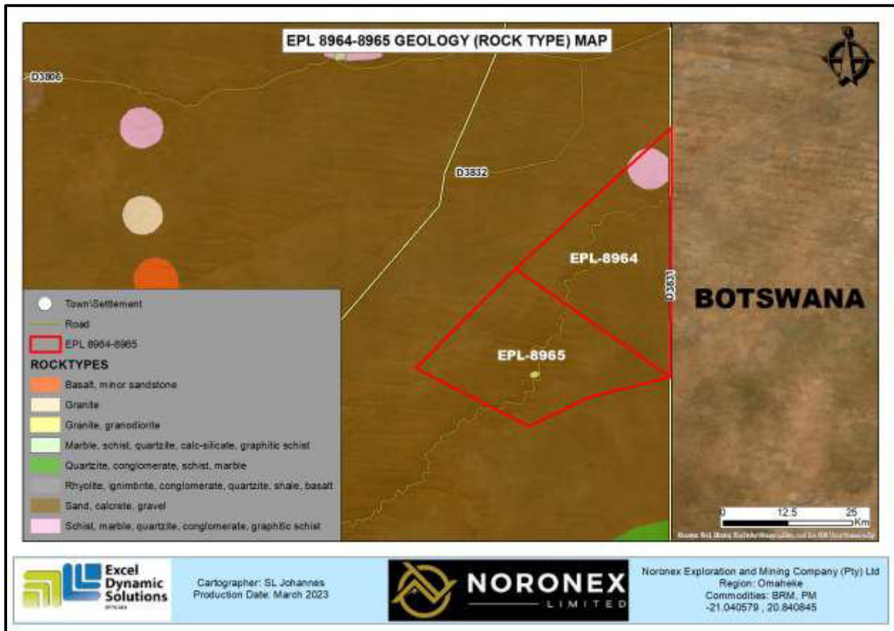
Figure 5: General Geology map - EPL 8964 – 8965
