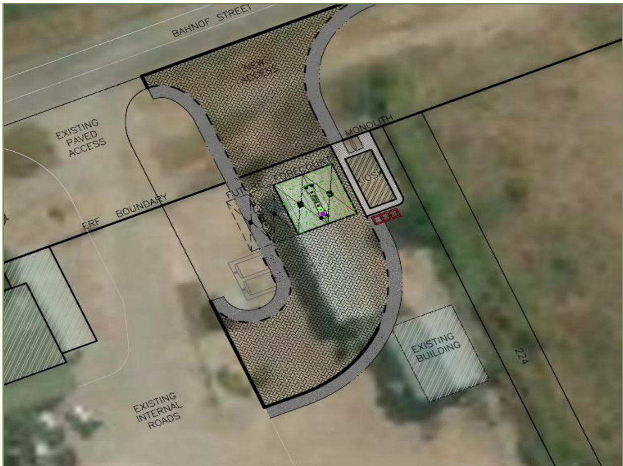
Figure 3. Installation layout
