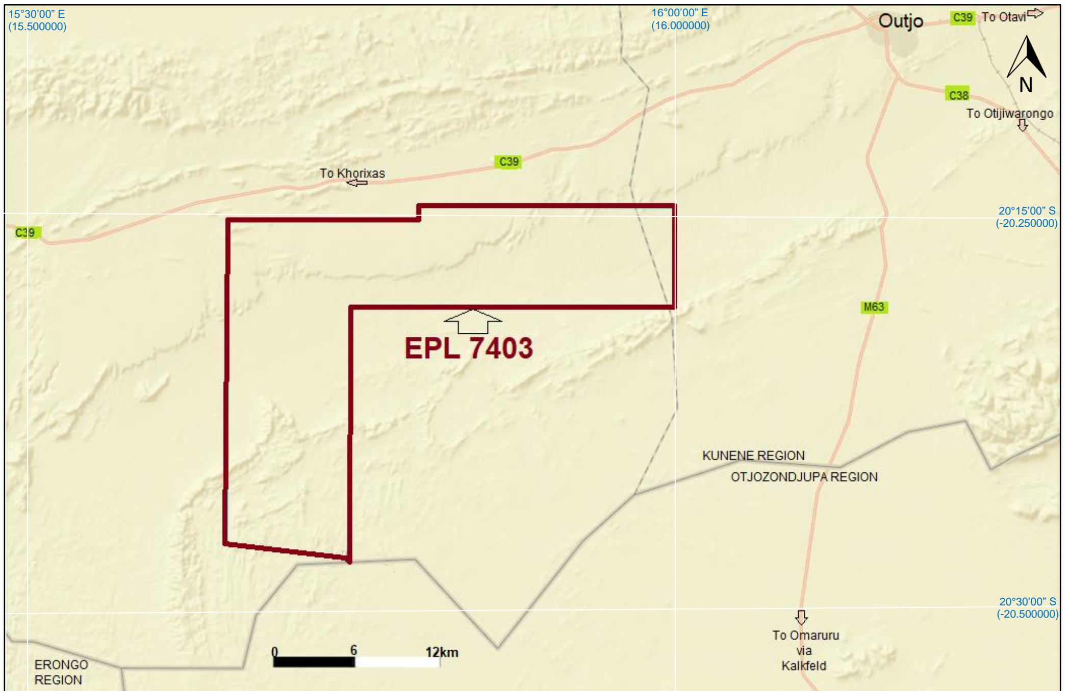
Figure 1.2: Detailed regional location of the EPL 7403 Area (Source: http://portals.flexicadastre.com/Namibia ).
