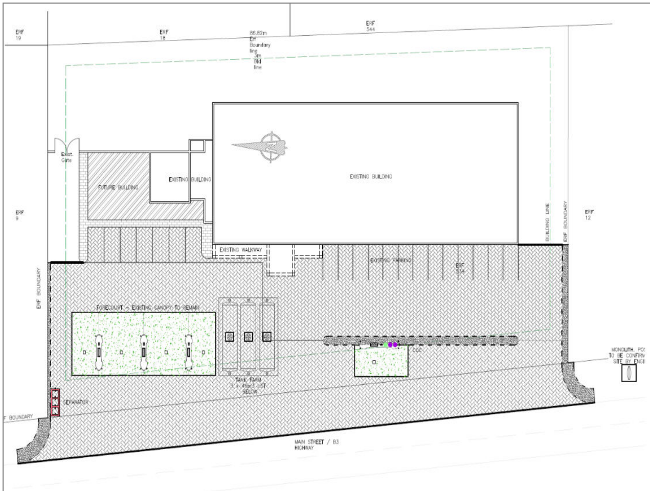
Figure 3. Installation layout
