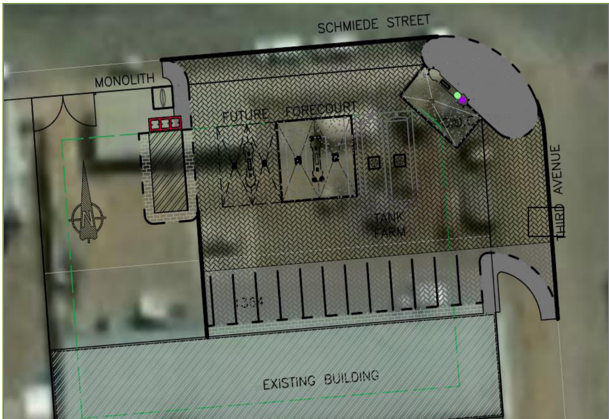
Figure 3. Installation layout
