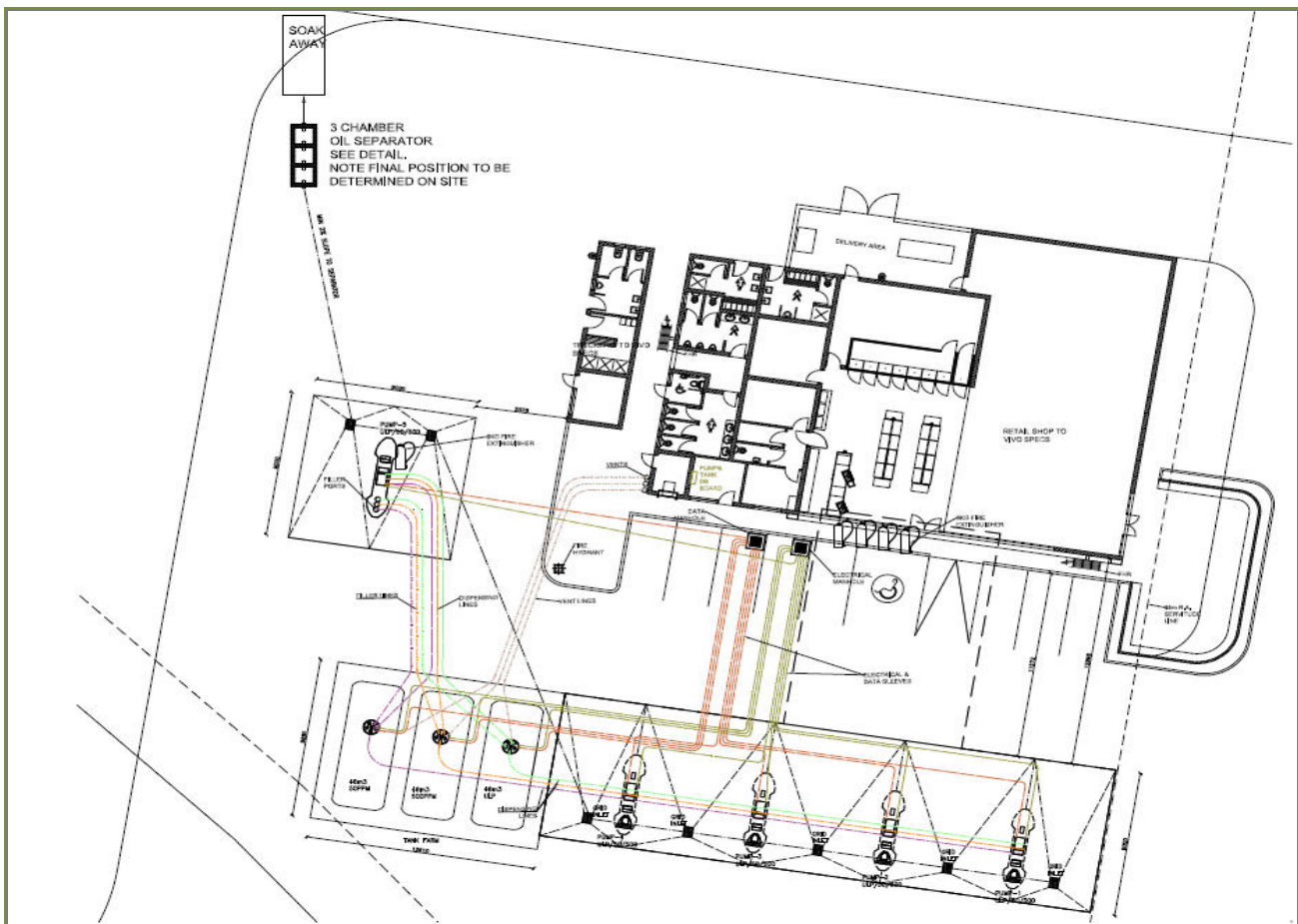
Figure 3. Layout of the facility
