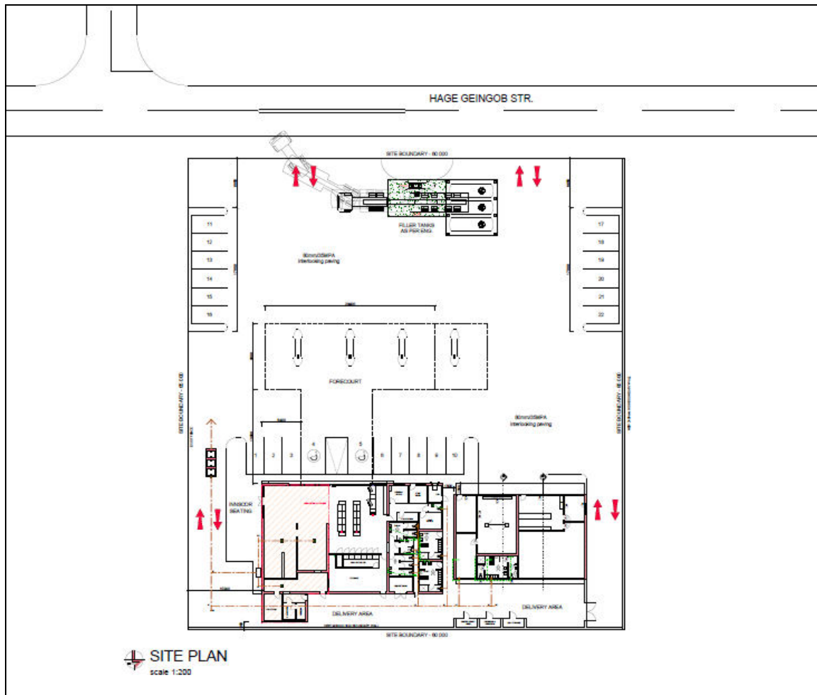
Figure 3. Installation layout
