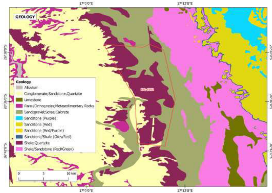
Figure 5: The geological map around the project area
