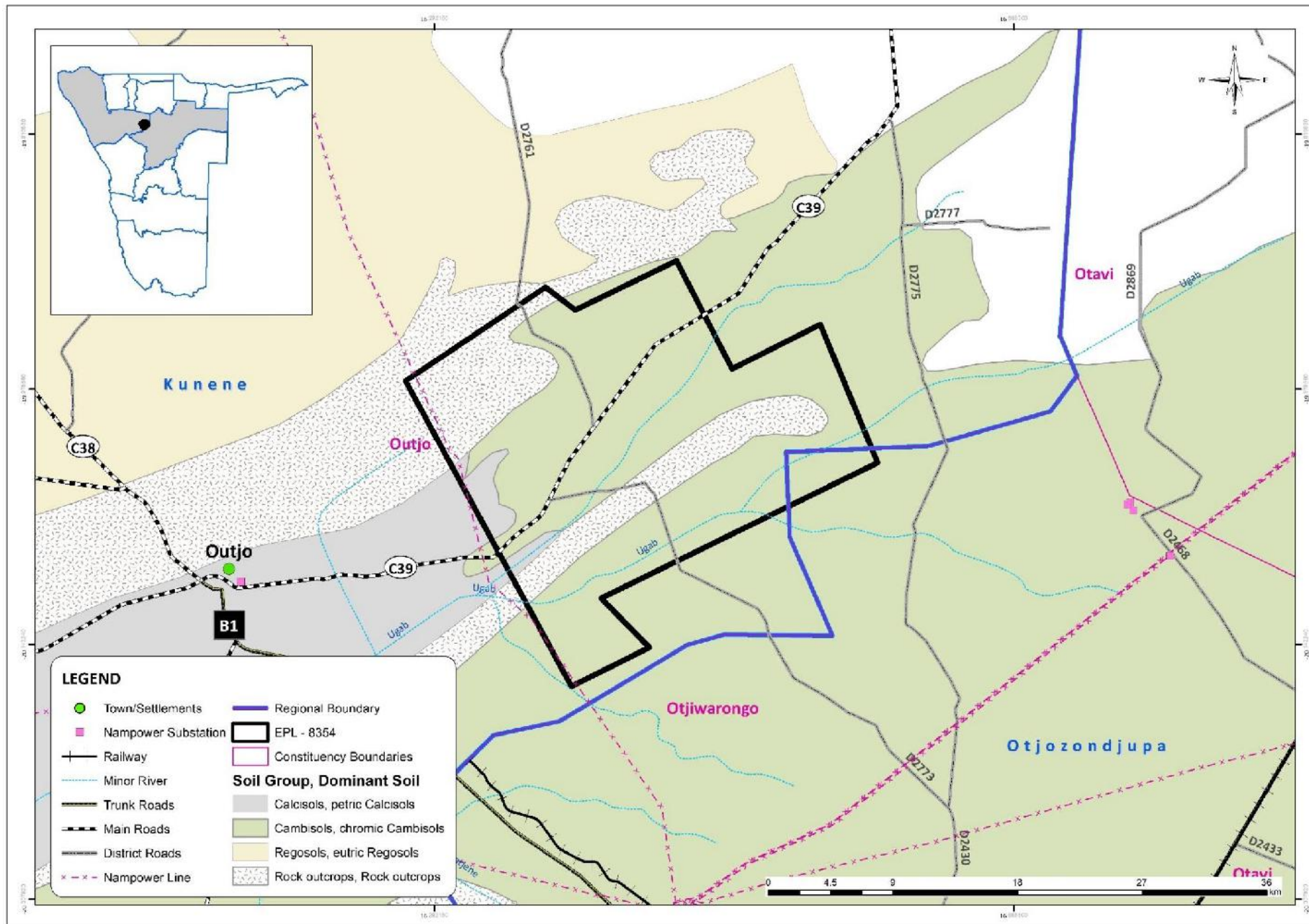
Figure 1.4: Soil found within and around the EPL No. 8354 area and related in infrastructure.
