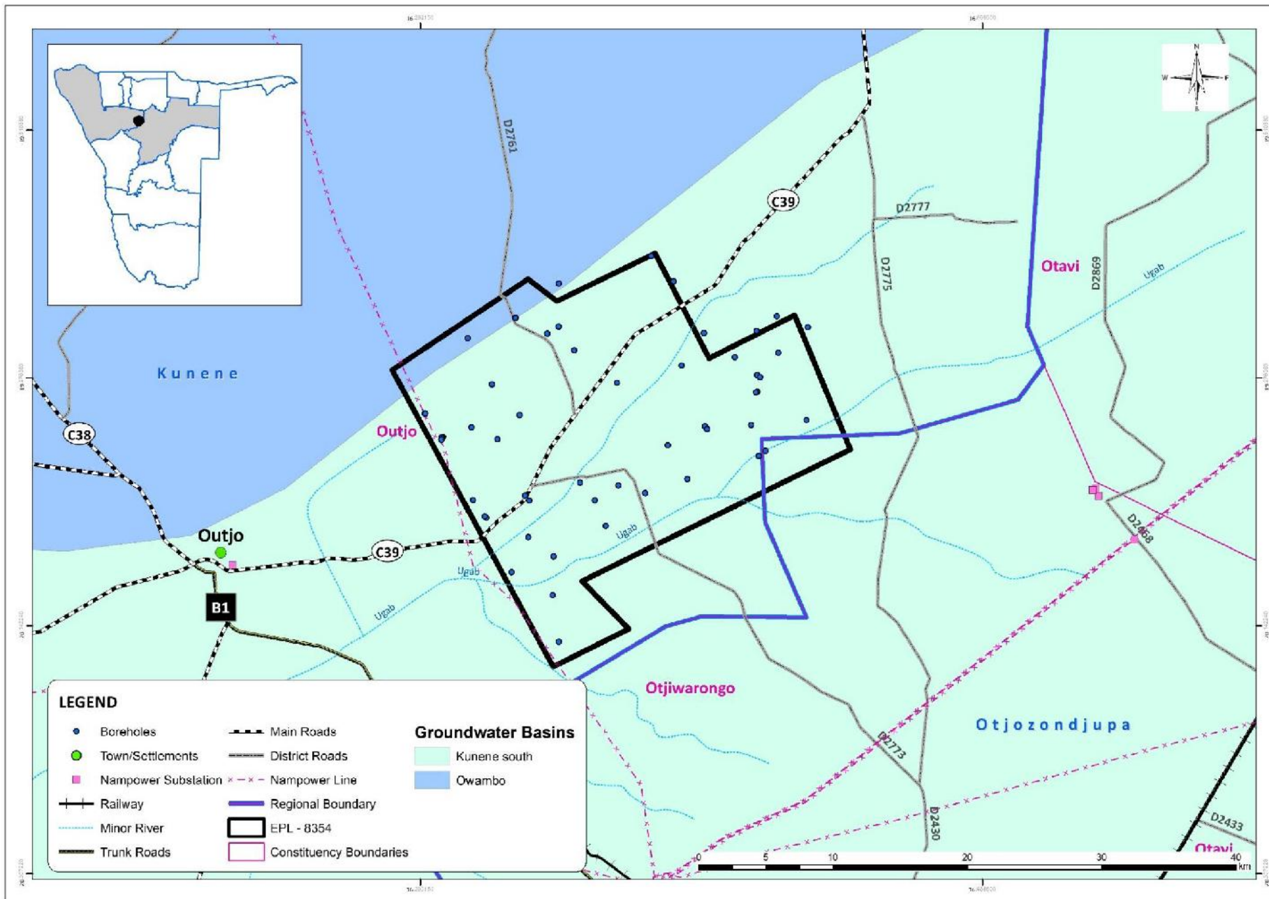
Figure 1.7: Groundwater found within and around the EPL No. 8354 area and related in infrastructure.
