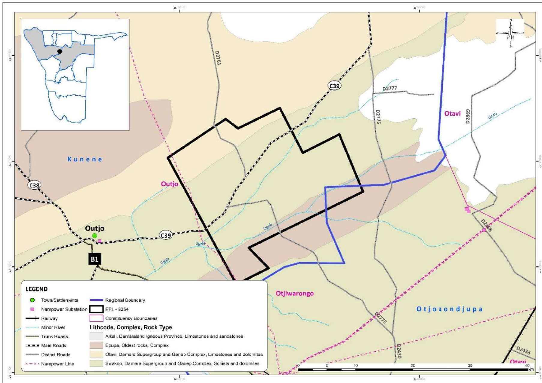
Figure 1.6: Rock types / solid geology found within and around the EPL No. 8354 area and related in infrastructure.
