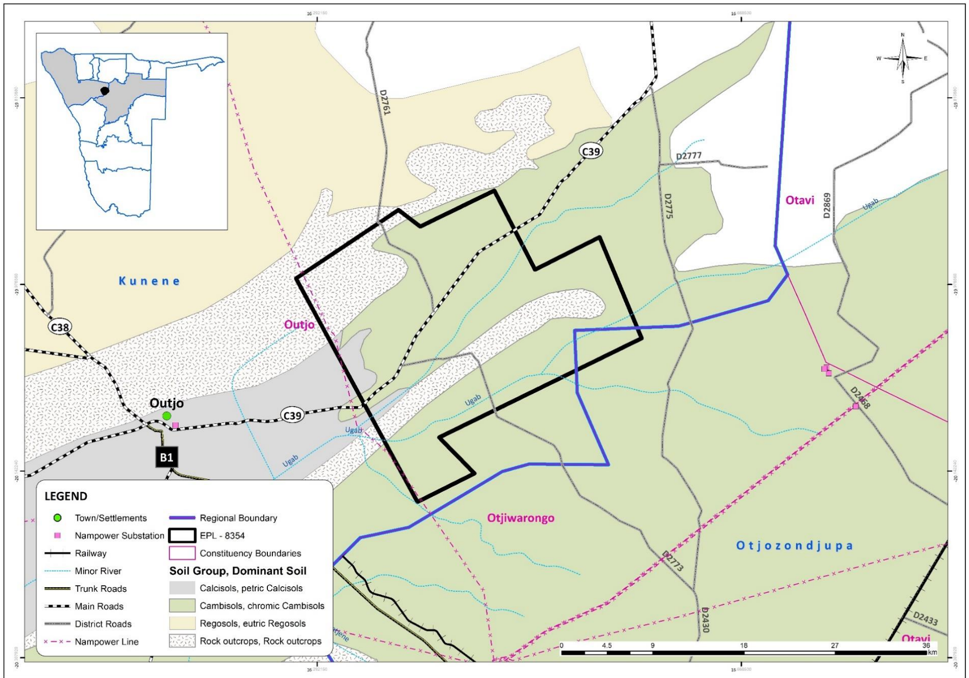
Figure 2:5: Simplified soil type map of the EPL 8354.
