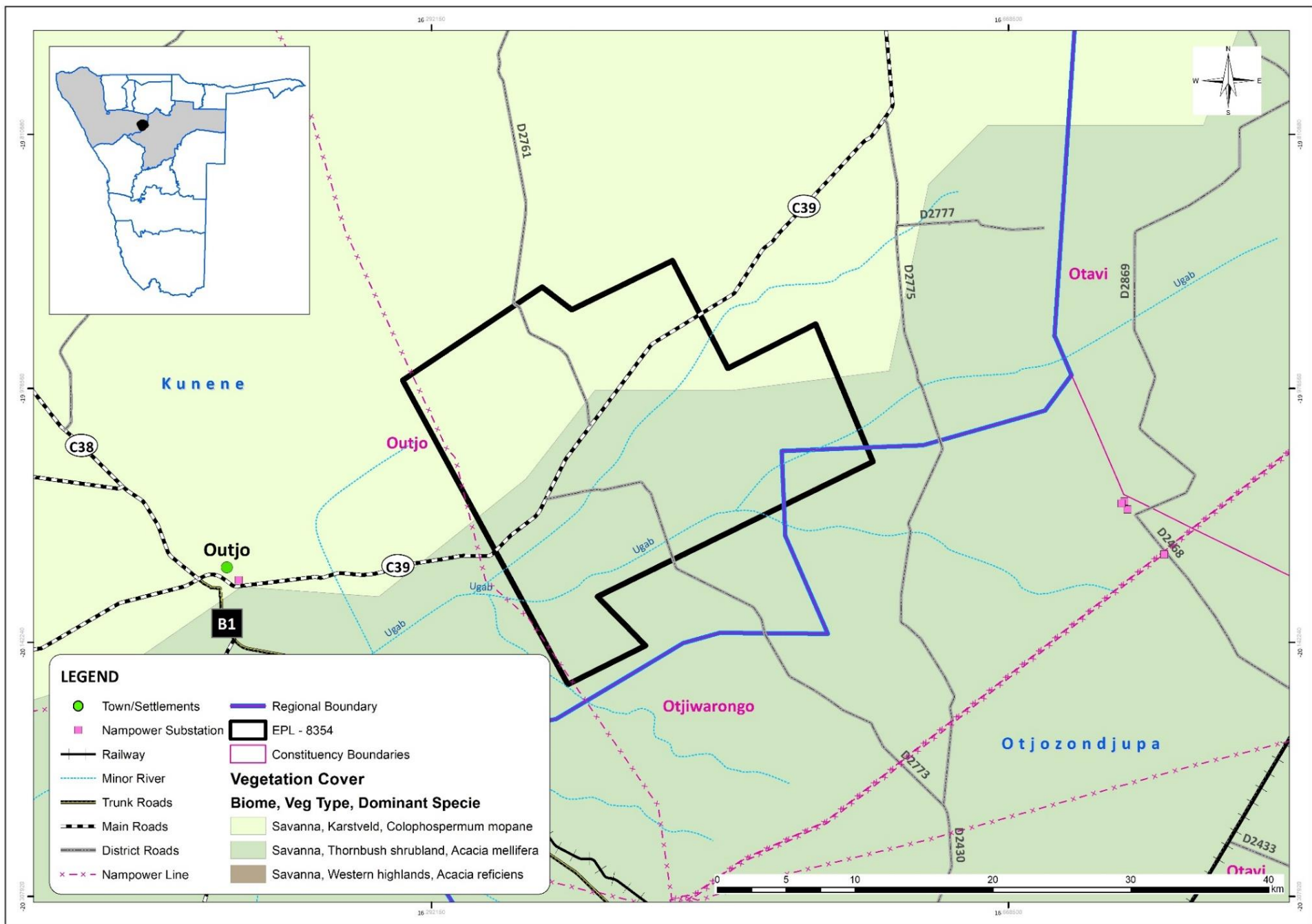
Figure 2:4: Vegetation map of the EPL 8354
