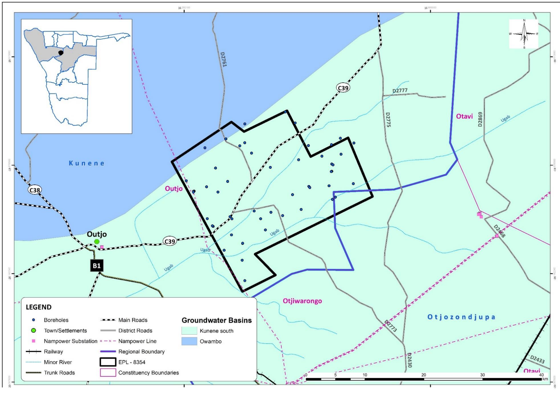
Figure 2:7 Simplified hydrogeological map of the EPL 8354
