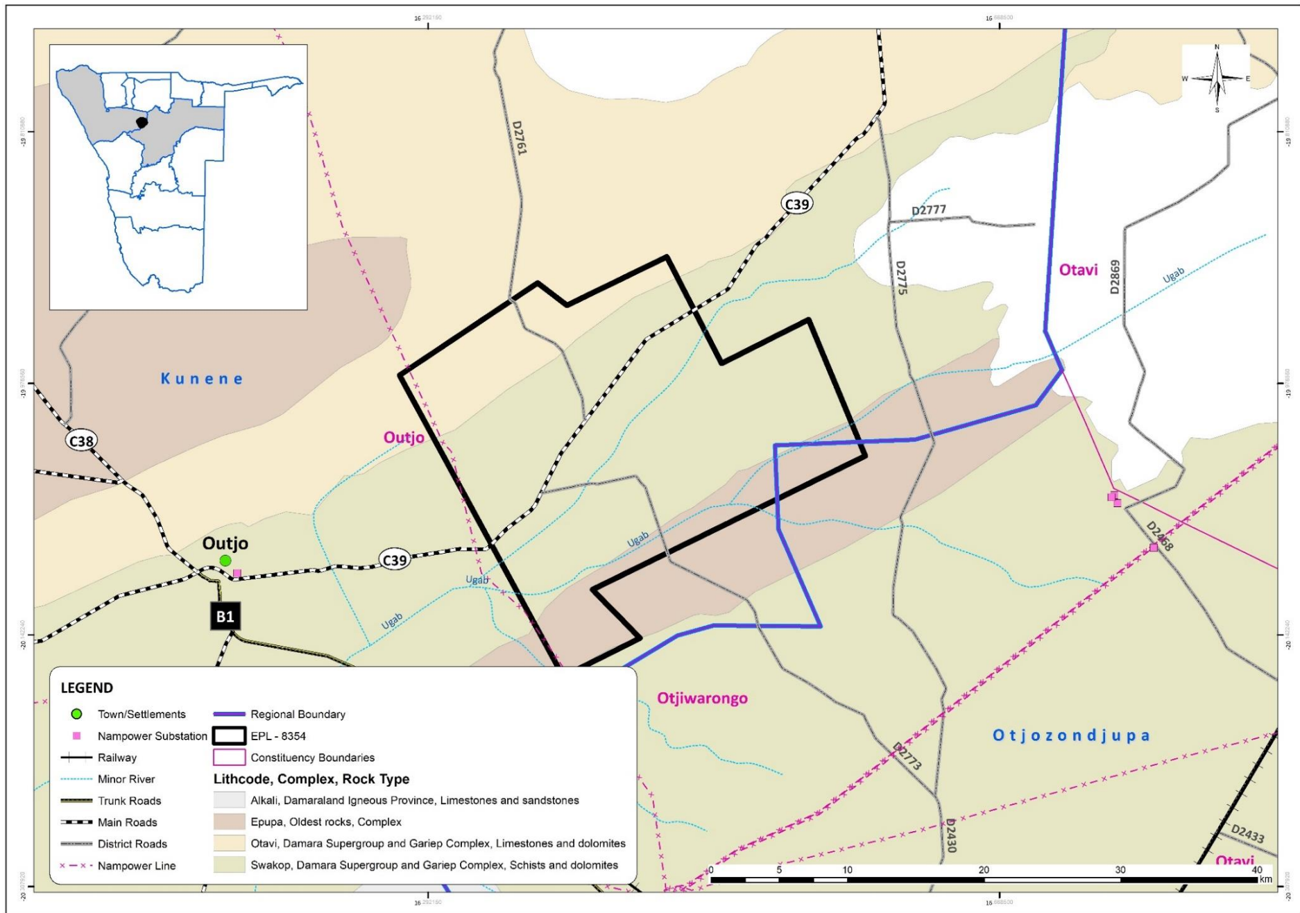
Figure 2:6 Simplified rock/geology map of the EPL 8354
