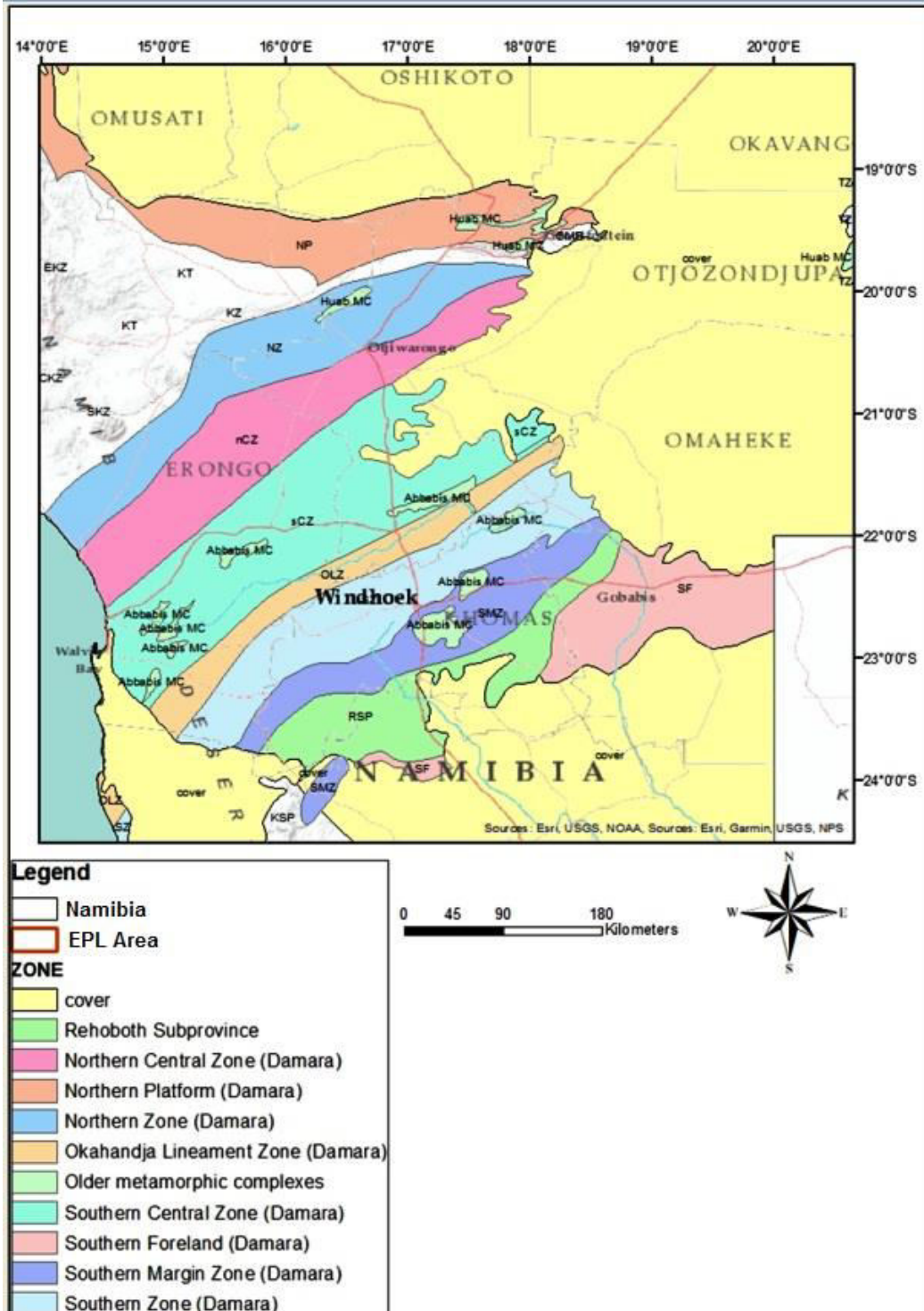
Fig. 22. Tectonic zones of the Damara orogenic belt. (Shape files are from the Geological Survey of Namibia). EPL 8742 is located in the northern central zone (nCZ) of the Damara belt.
