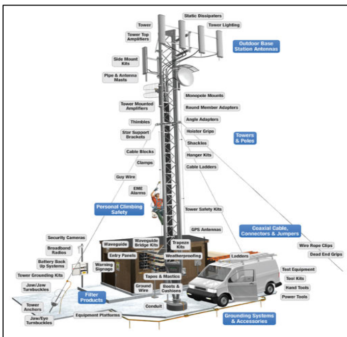
Figure 5: Typical telecommunication towers structure and form (visual puproposes only)
